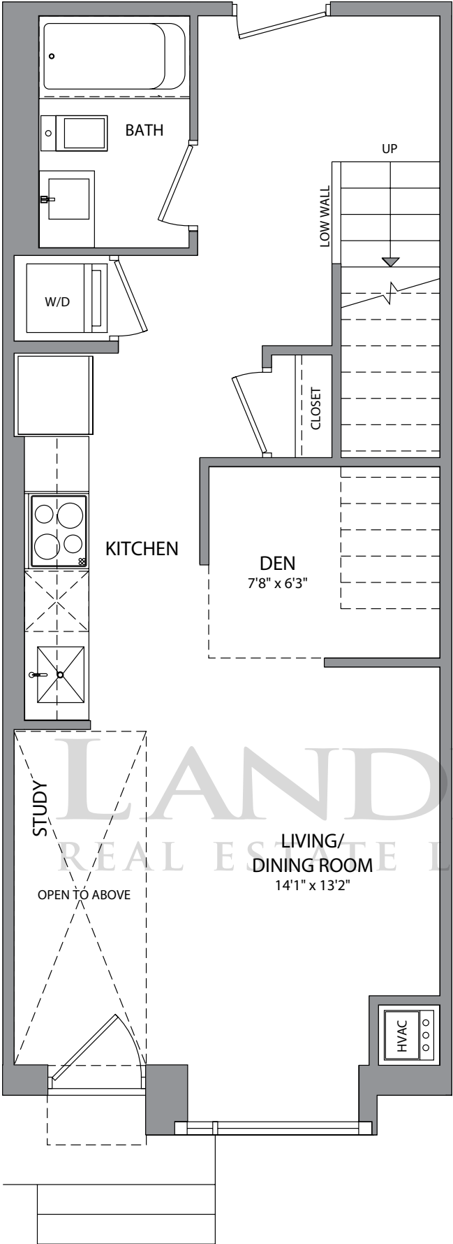
GROUND FLOOR LEVEL 1
