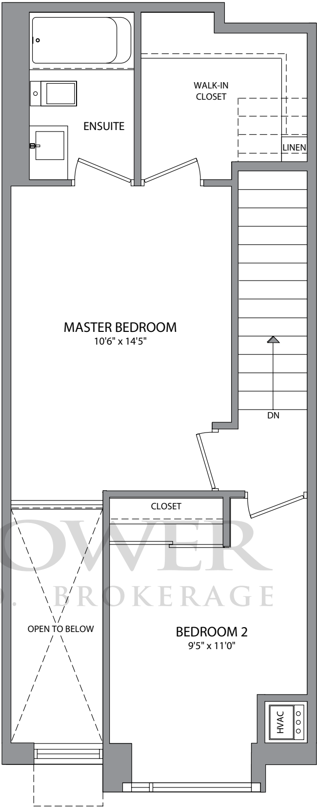
SECOND FLOOR LEVEL 2
