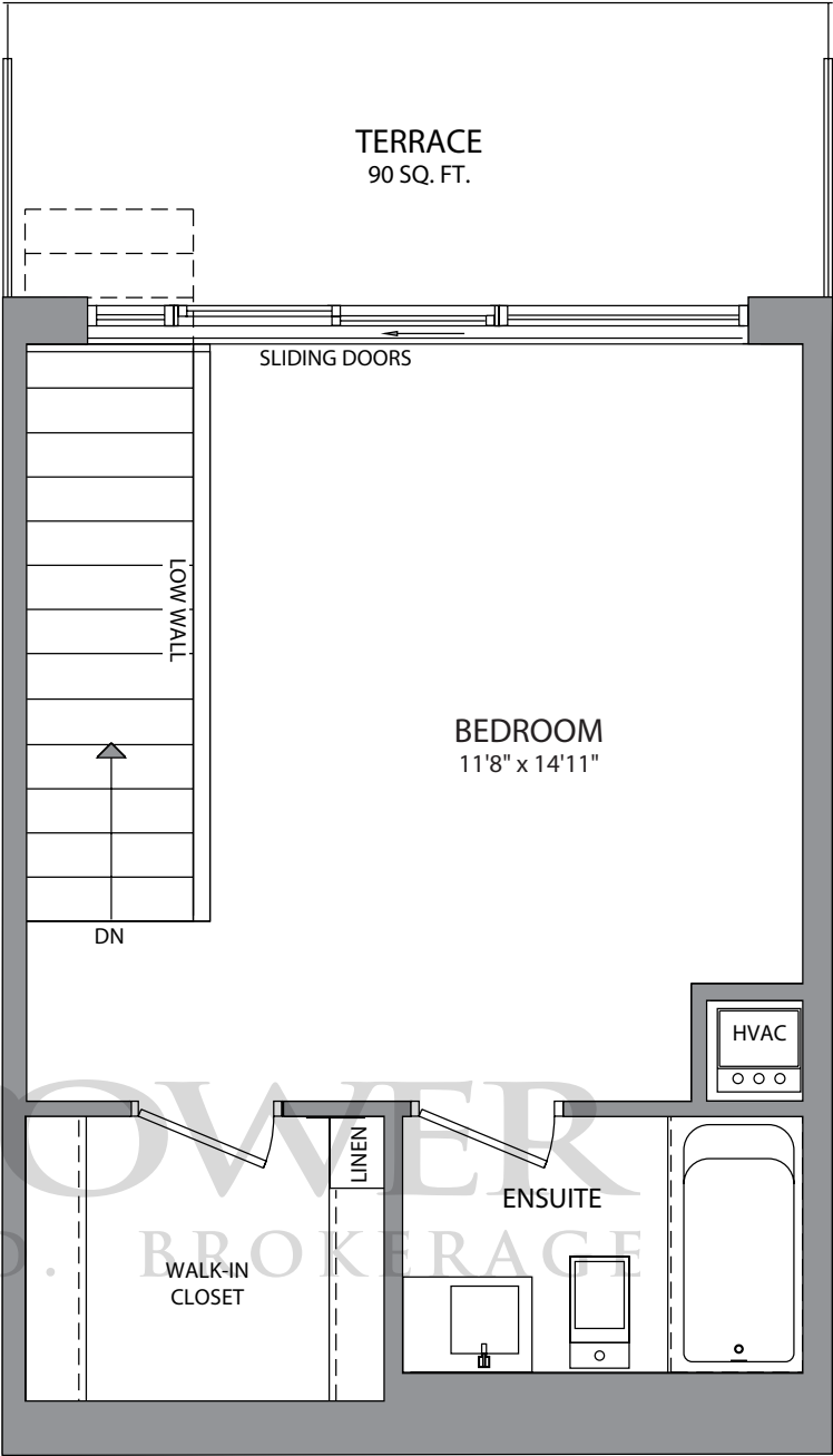
FIFTH FLOOR LEVEL 2
