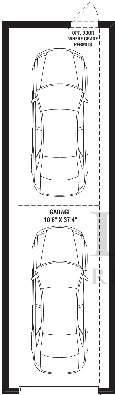
DETACHED GARAGE
