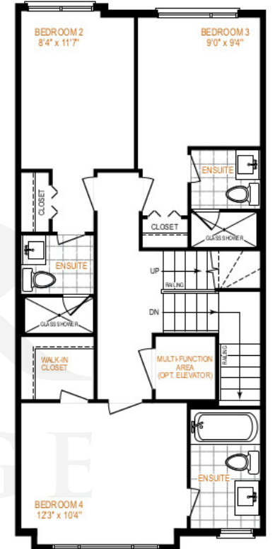
Alt. Upper level (4 Bedroom option with lower level laundry)
