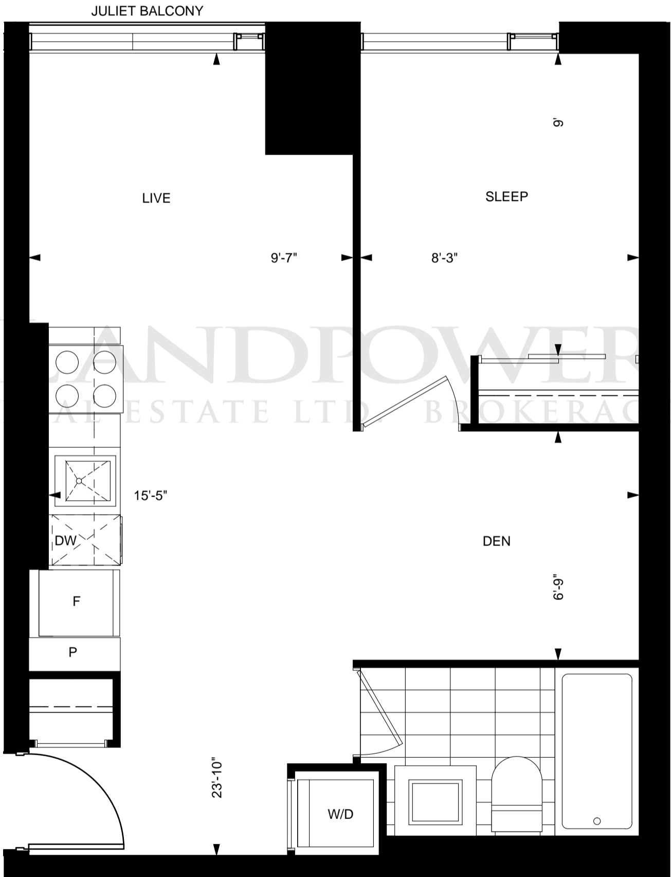
3rd-5th Floors
