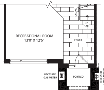
PARTIAL- GROUND FLOOR PLAN ELEVATION 'B'
