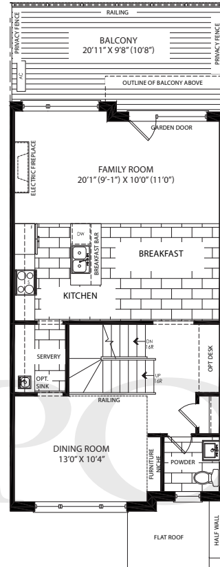
SECOND FLOOR PLAN ELEVATION 'A'
