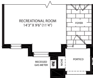
PARTIAL- GROUND FLOOR PLAN ELEVATION 'B'
