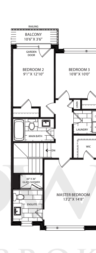
THIRD FLOOR PLAN ELEVATION 'A'
