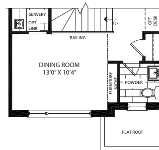
PARTIAL- SECOND FLOOR PLAN ELEVATION 'B'
