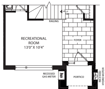
PARTIAL- GROUND FLOOR PLAN ELEVATION 'B'
