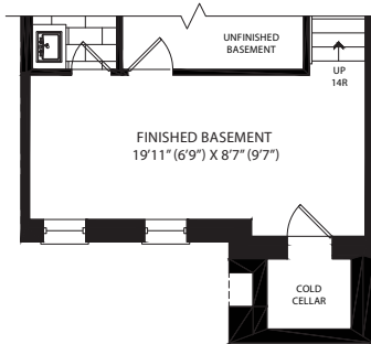
PARTIAL- BASEMENT FLOOR PLAN ELEVATION 'B'
