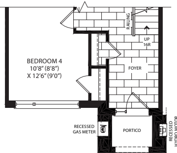
PARTIAL-OPT. GROUND FLOOR PLAN BEDROOM W/ BATH ELEVATION 'B'
