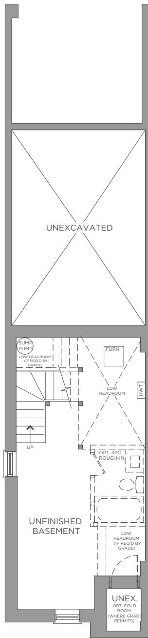
BASEMENT ELEVATION A & B
