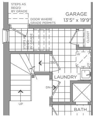
OPT. FIRST FLOOR
