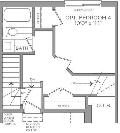
FIRST FLOOR BEDROOM 4
