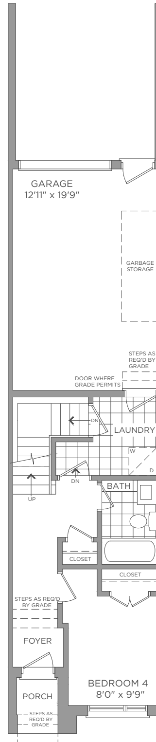
OPT. FIRST FLOOR ELEVATION A
