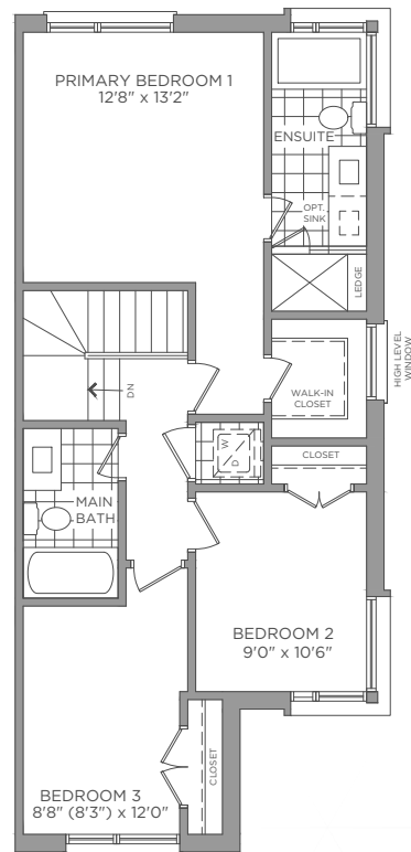
OPT. THIRD FLOOR 3 BEDROOM WITH LAUNDRY
