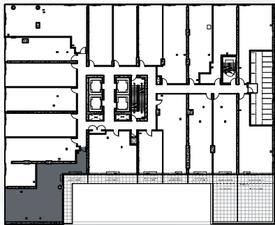
TYPICAL FLOORS 3-7
