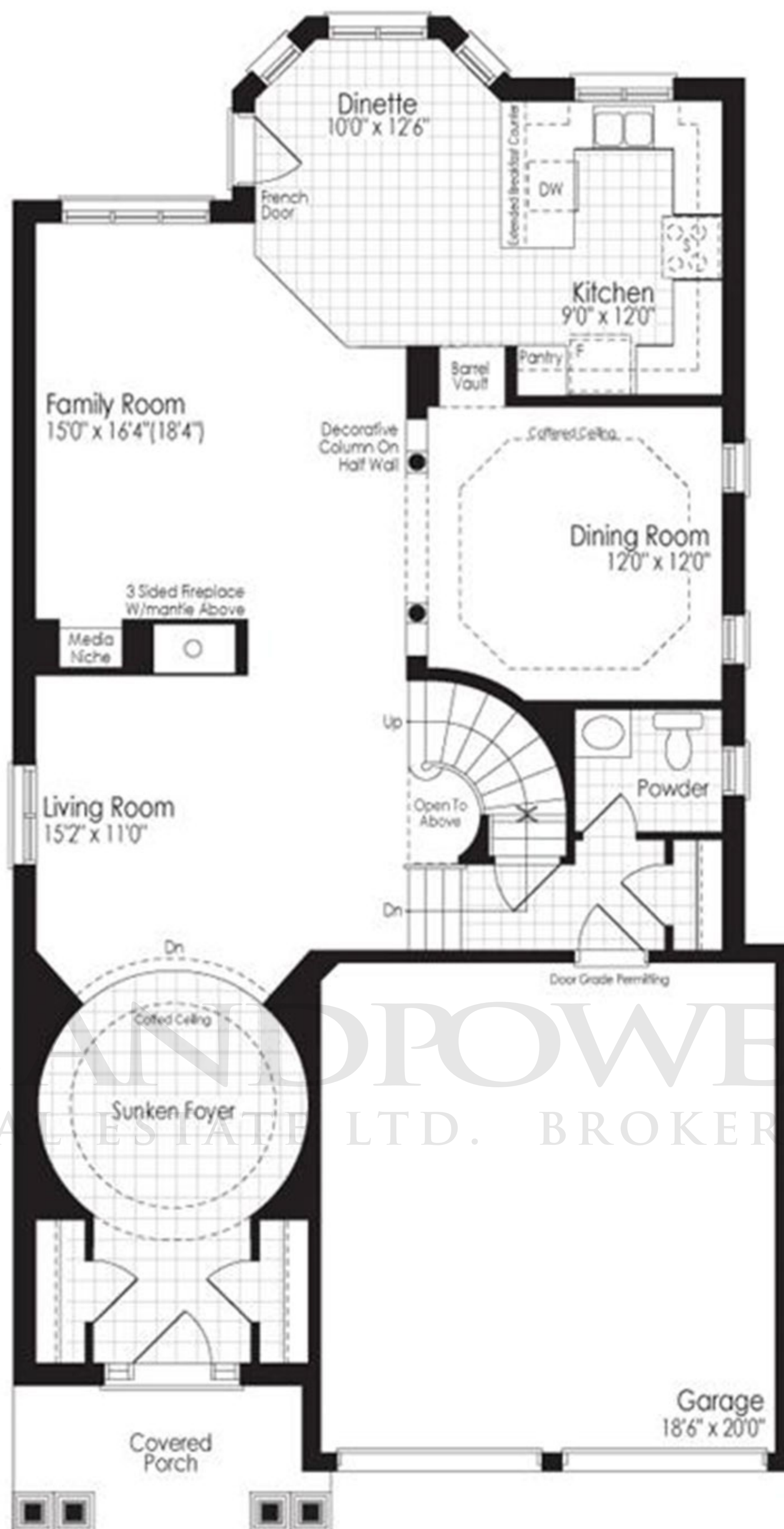
Ground Floor Plan Elev. A
