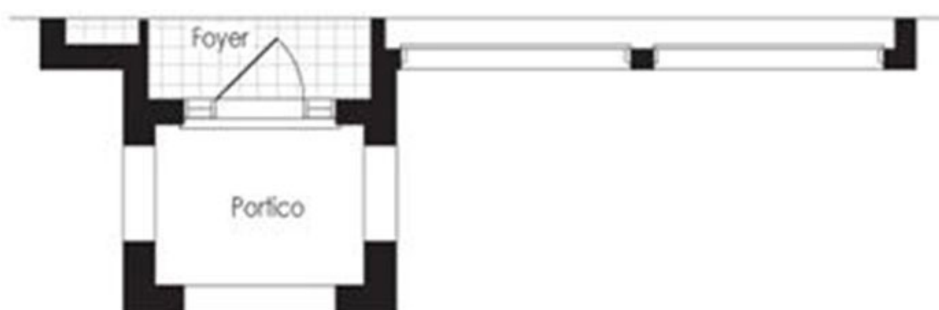
Ground Floor Plan, Elev. B
