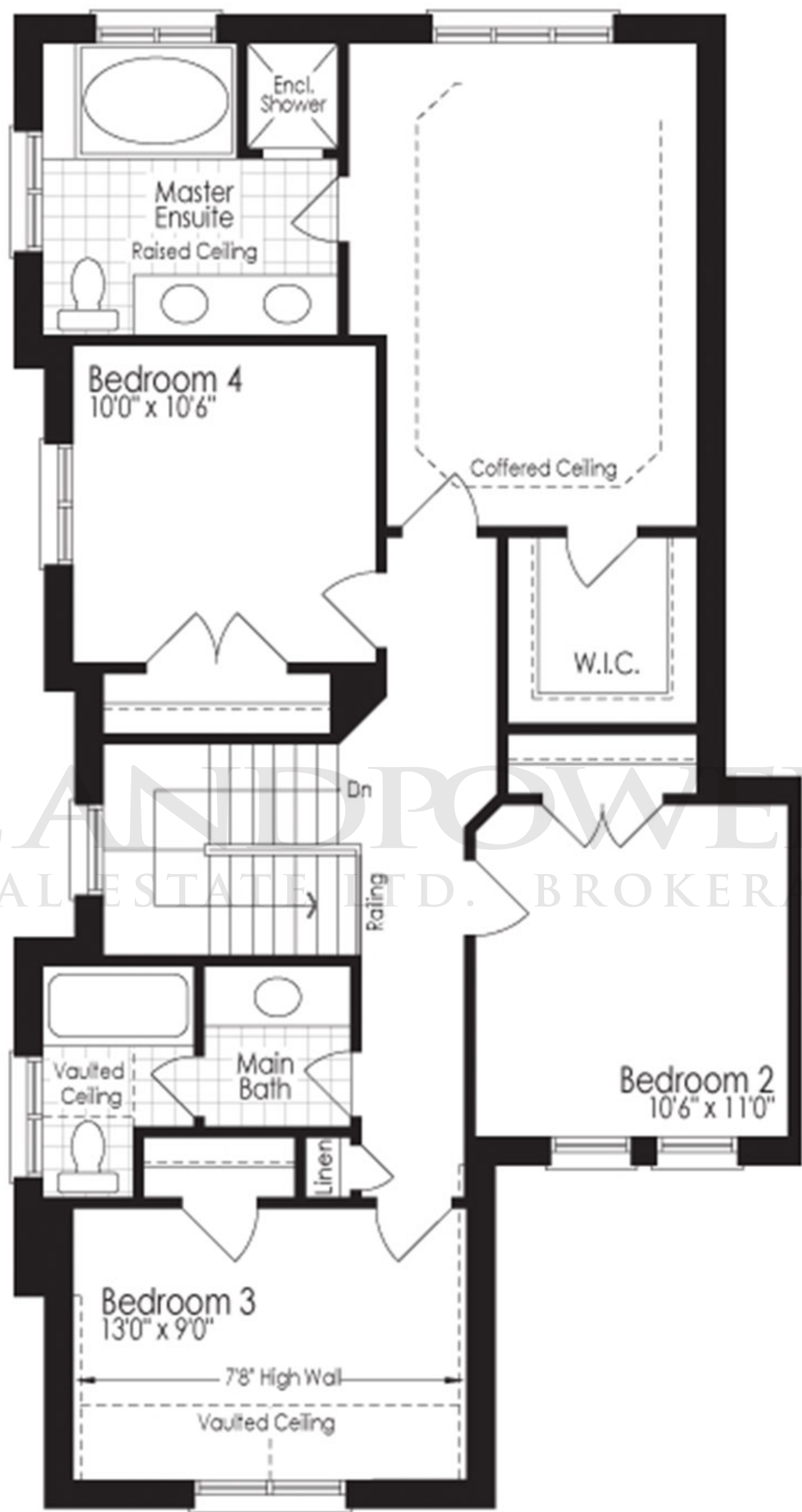
Corner Upgrade Second Floor Plan 'B'
