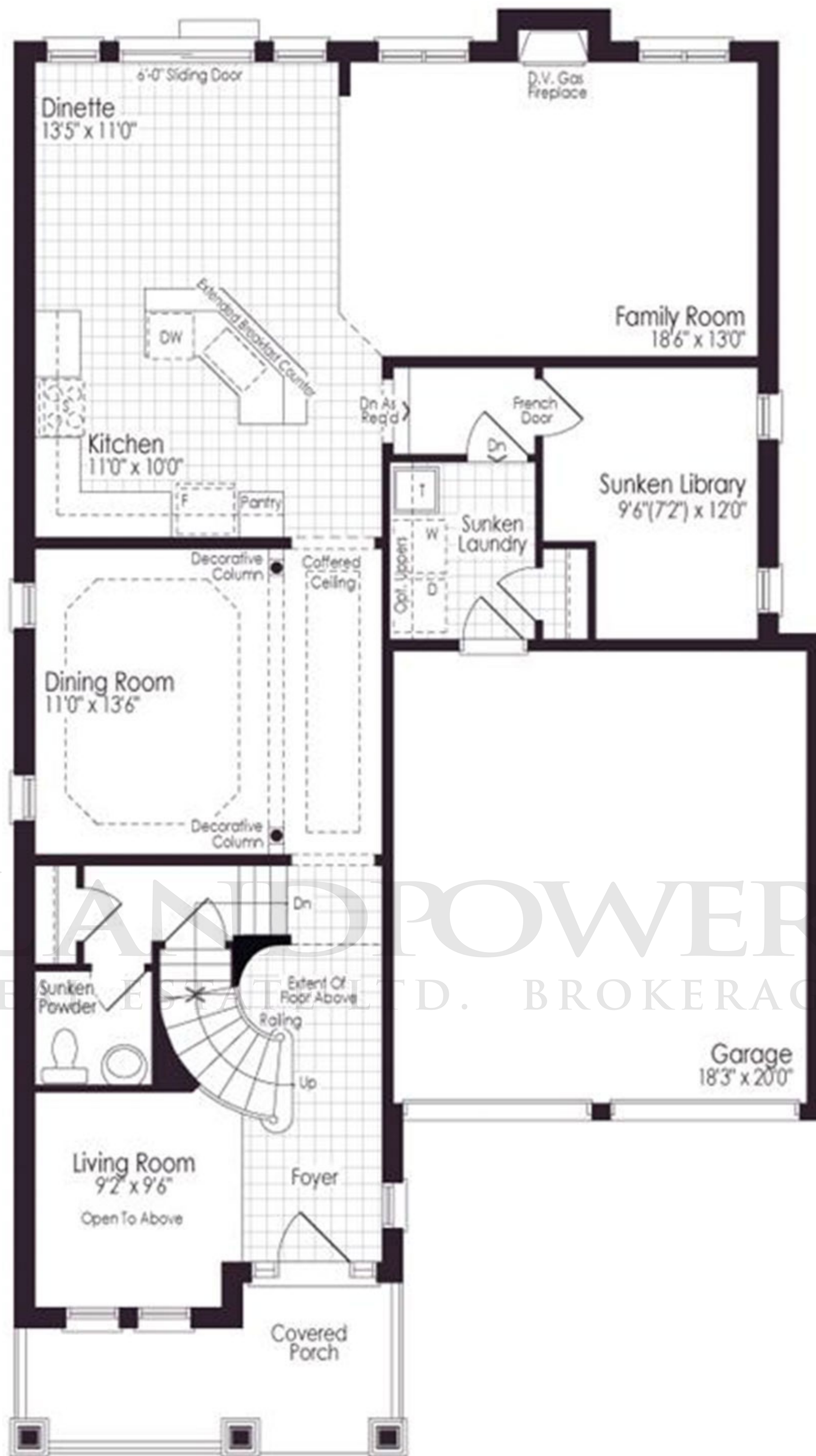
Ground Floor Plan Elev. A
