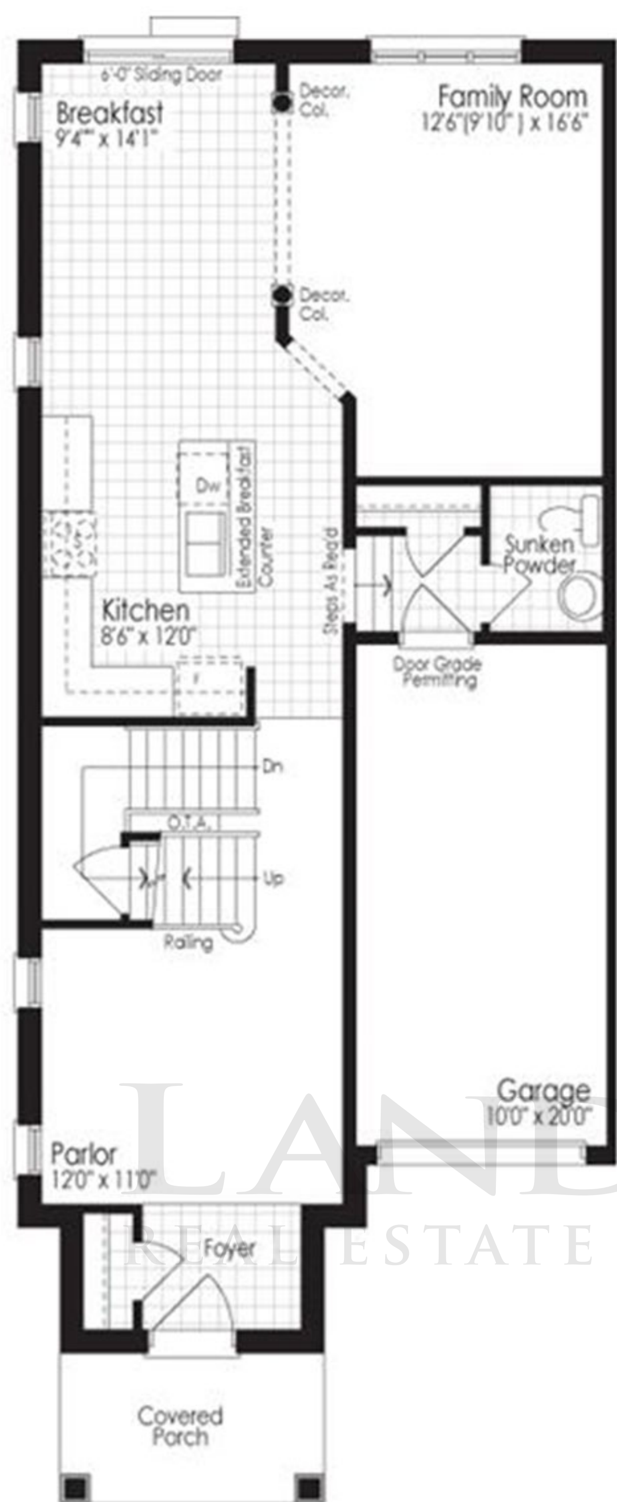
Alt. Ground Floor Plan 'A' Alt. Ground Floor Plan 'B'
