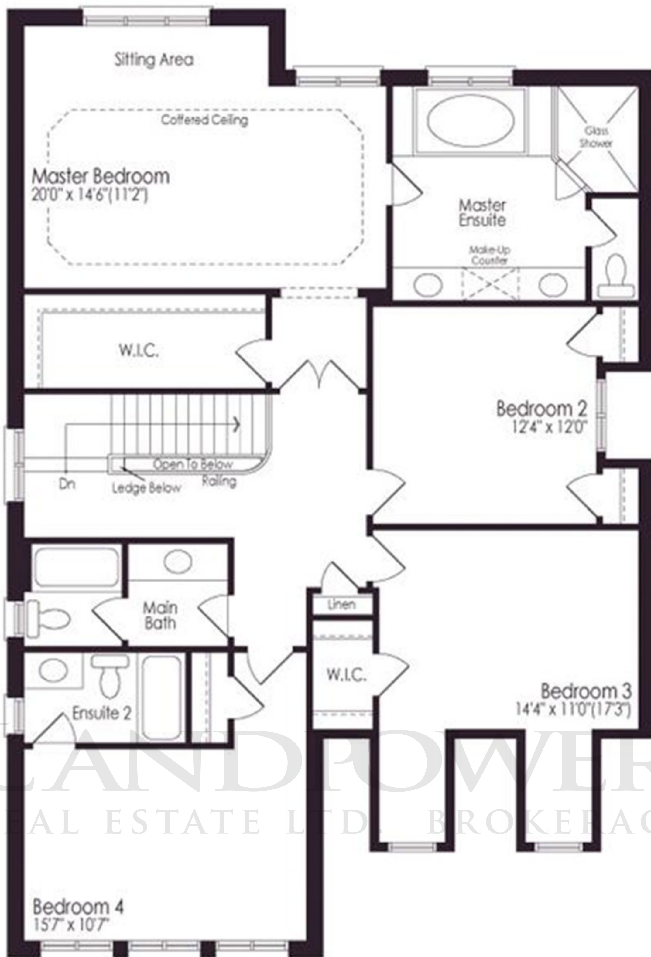
Second Floor Plan Elev. A
