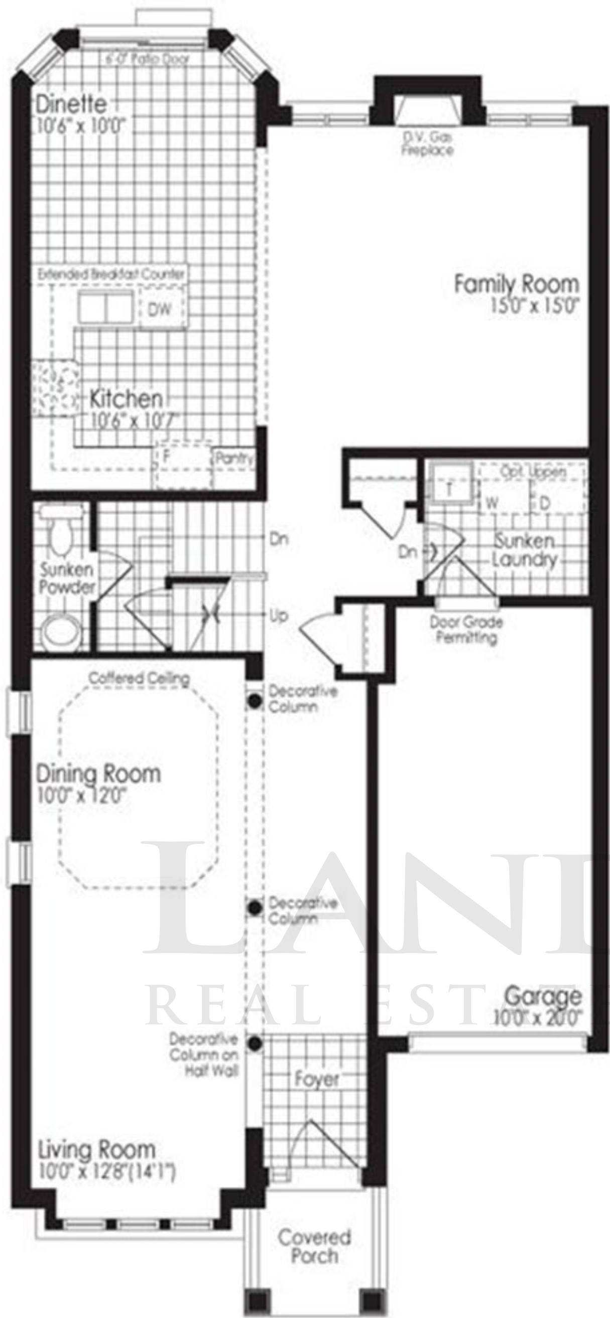
Ground Floor Plan, El. 'A'
