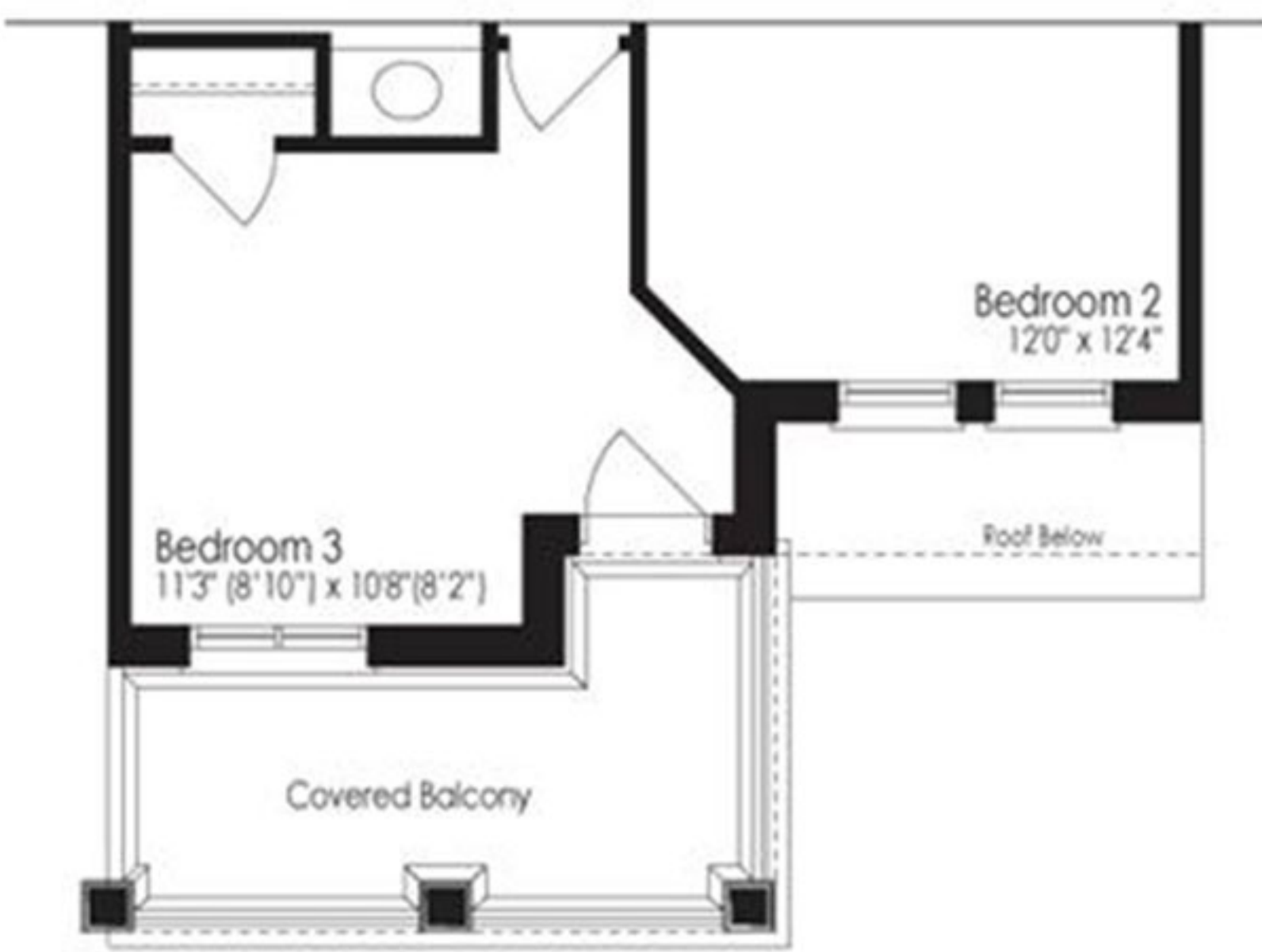
Partial Second Floor Plan Elev. B
