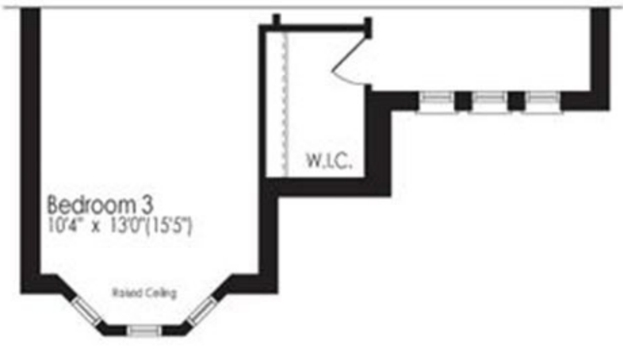
Second Floor Plan, El. 'B'
