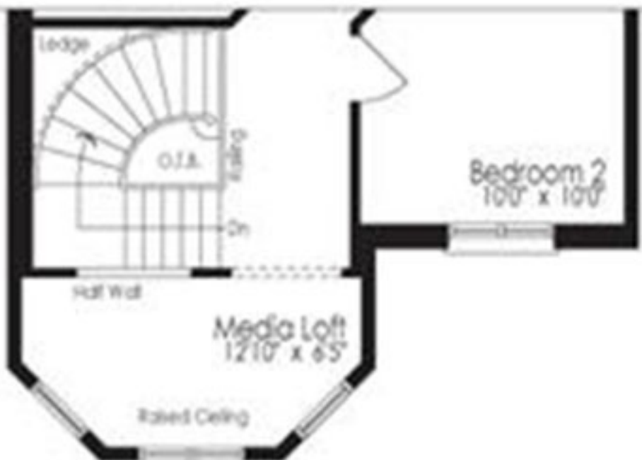
Second Floor Plan 'C'
