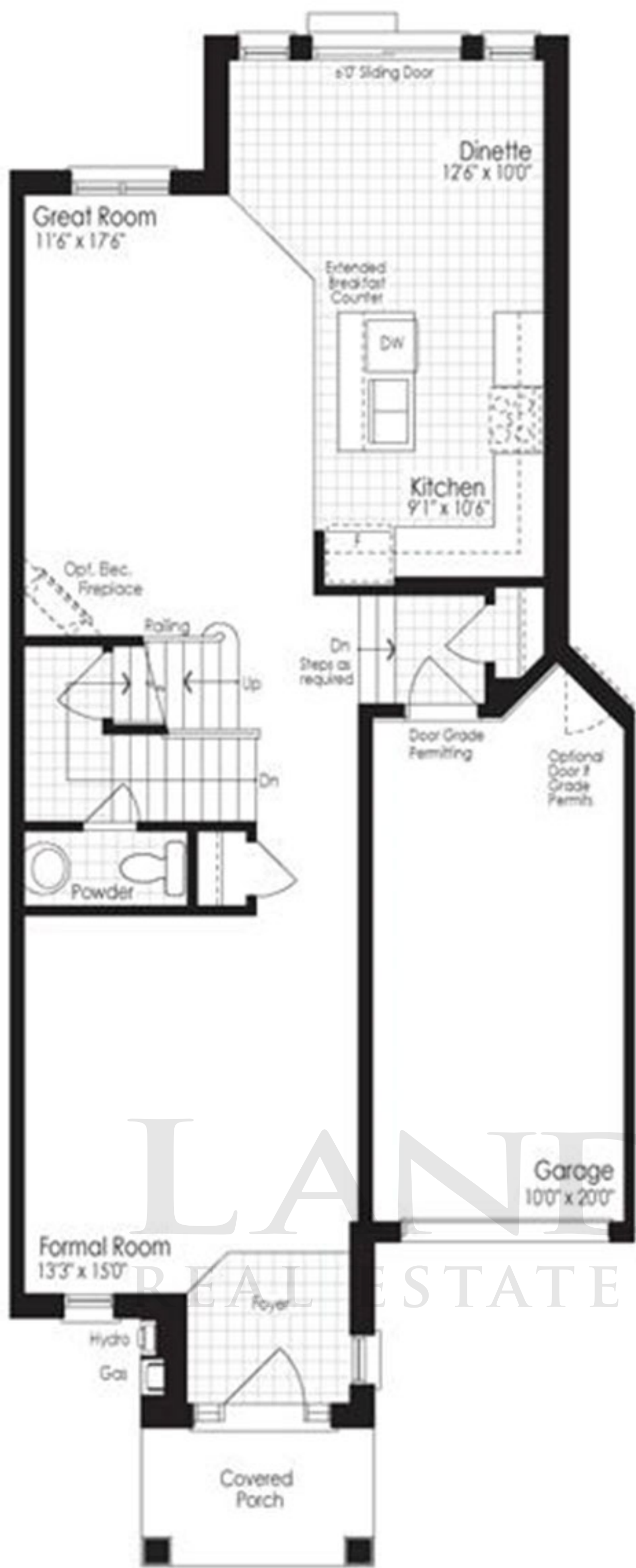
Ground Floor Plan Elev. A
