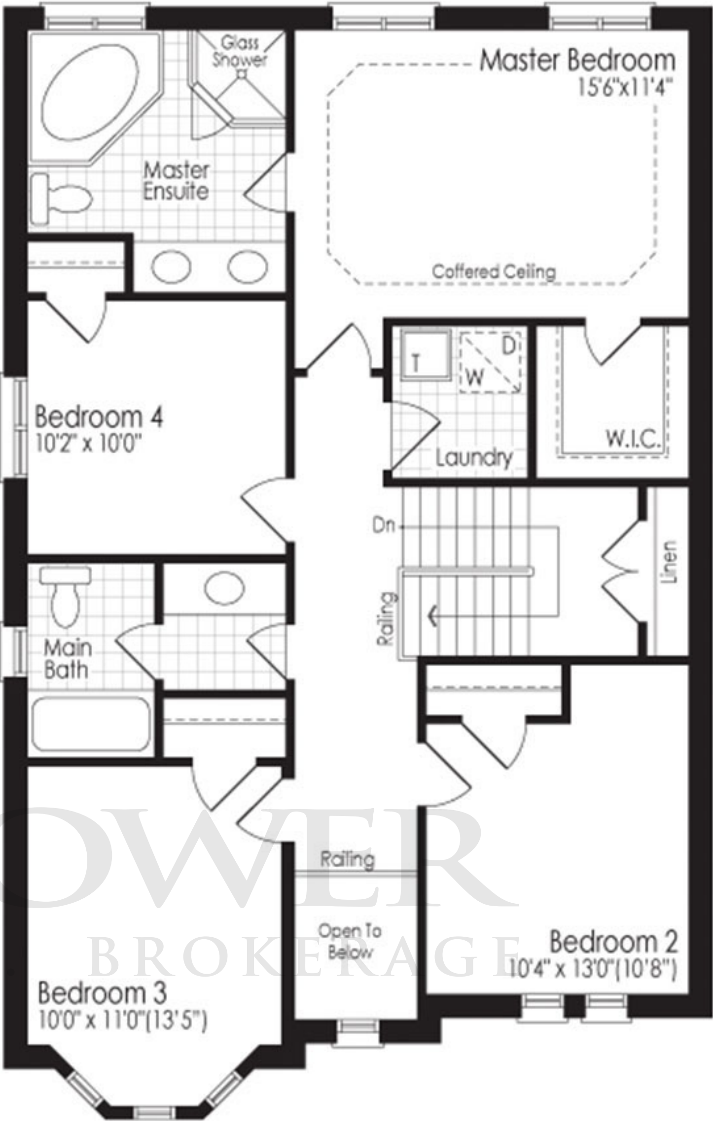
Second Floor Elev. B
