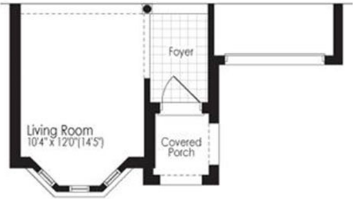
Ground Floor Plan, El. 'B'
