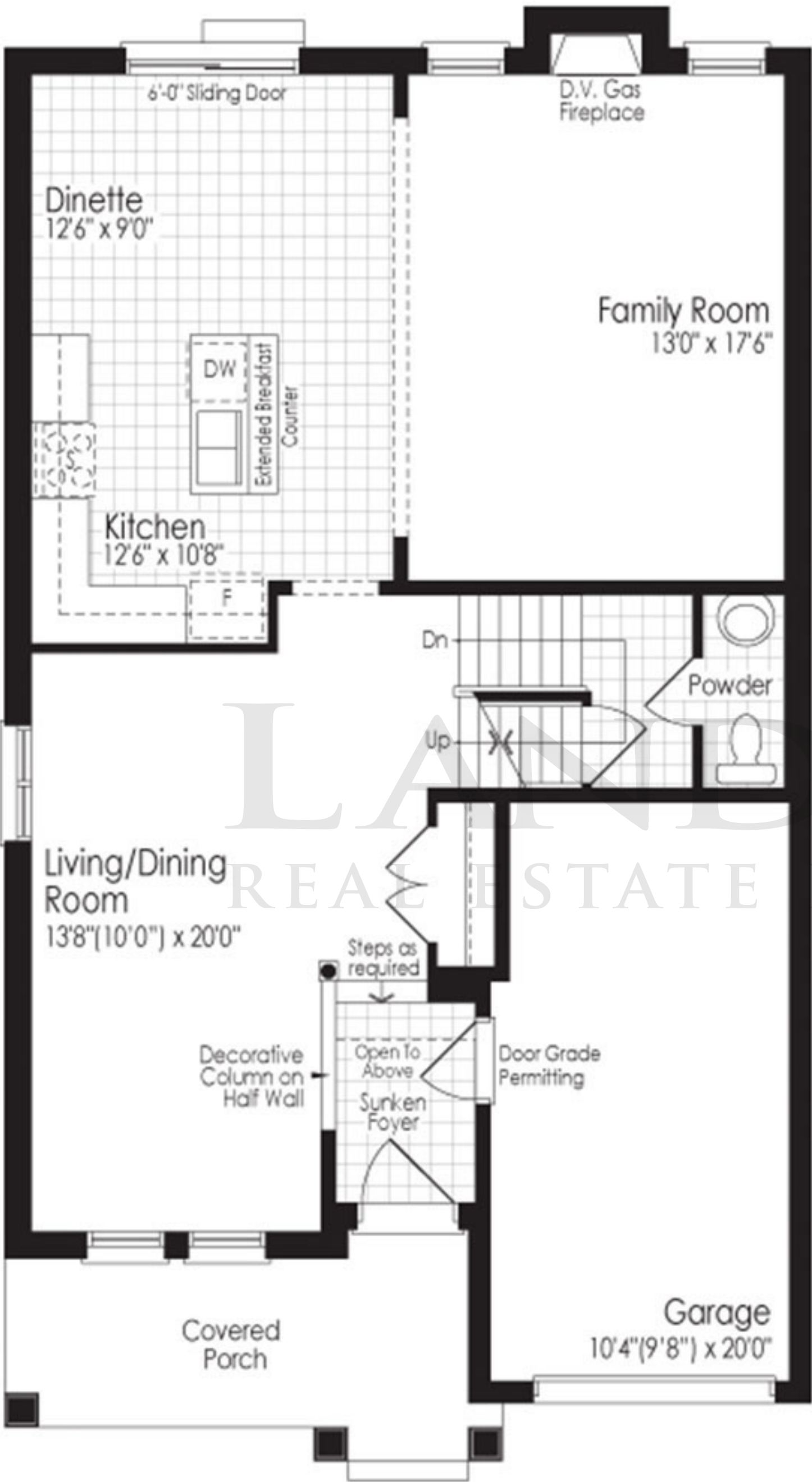
Ground Floor Plan Elev. A & B
