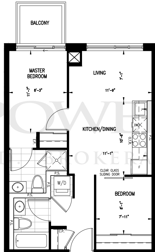
UNITS 904, 905, 1004, 1005, 1103, 1104, 1203, 1204
