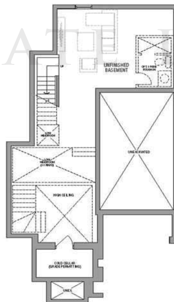
BASEMENT
