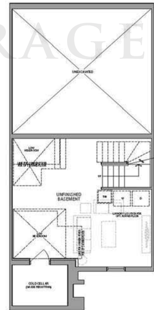
BASEMENT
