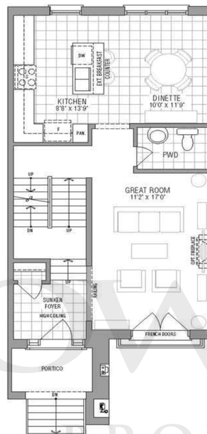
MAIN FLOOR
