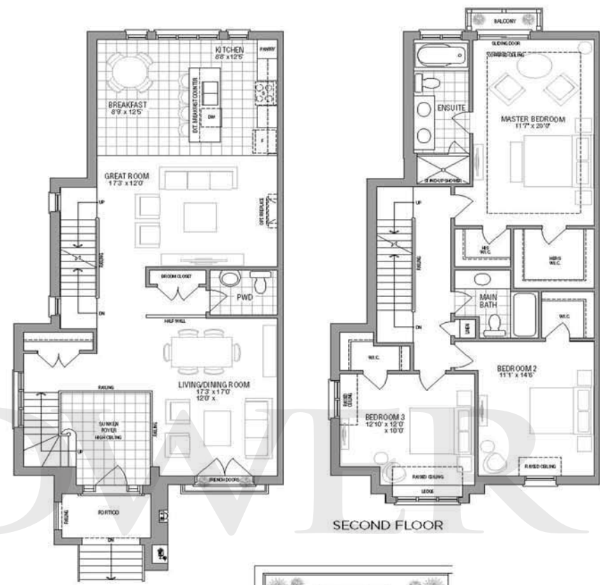
MAIN FLOOR
