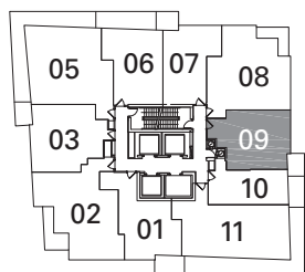
LEVELS 19/31/43 BALCONY 47 SQ. FT. TYPICAL LOWER RECESSED FLOOR
